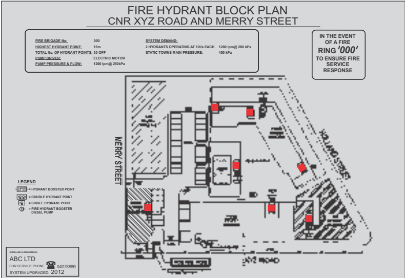
BLOCK PLANS (As per your requirement)
